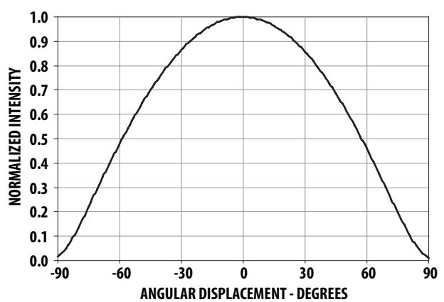
Figure 11. Radiation Pattern
