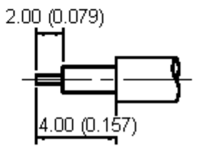
Stripping Dimension Dimensions : Millimetres (Inches)
