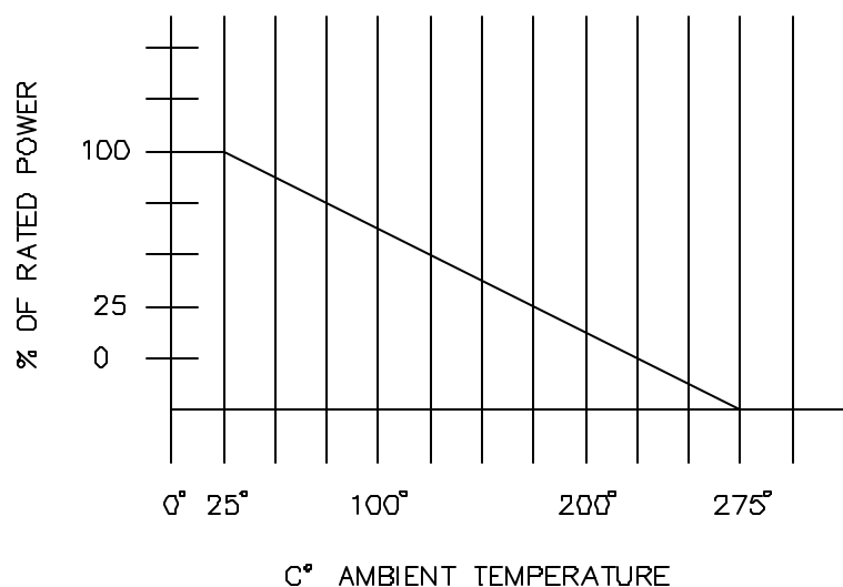
DERATING CURVE
