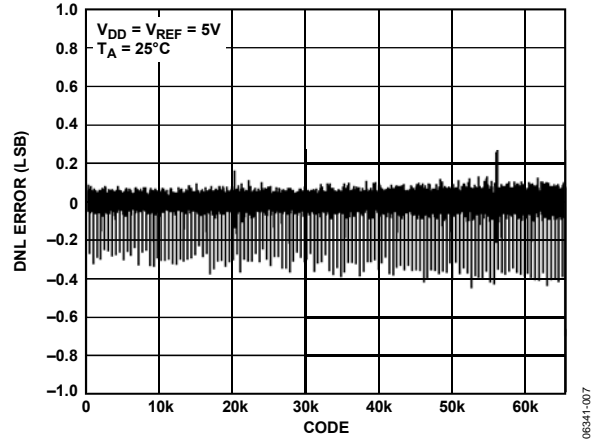
Figure 11. DNL AD5665, External Reference
