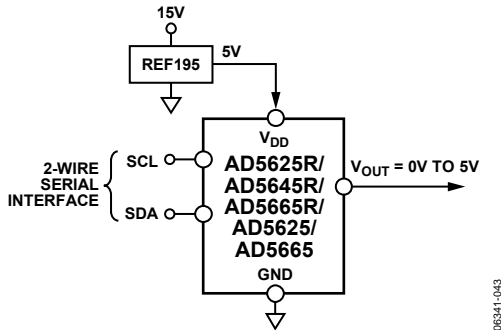
Figure 71. REF195 as Power Supply to the AD56x5R/AD56x5
