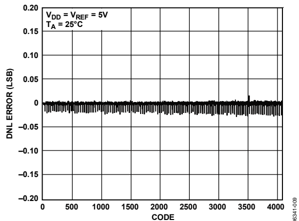
Figure 13. DNL AD5625, External Reference
