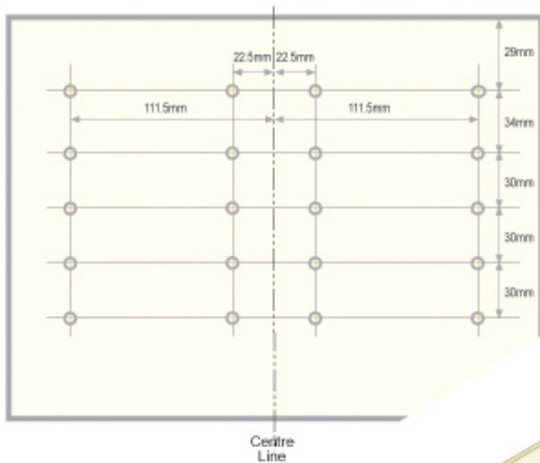
Matrix of strengthened mounting points Dimensions assume 3mm wall thickness of box
