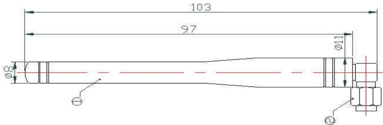
Figure 1 right-angled SMA
