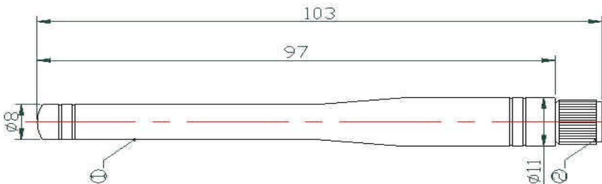
Figure 3 straight SMA
