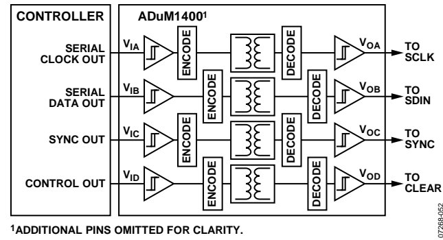
Figure 58. Isolated Interface
