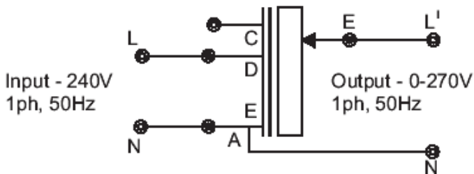
Connection Arrangement
