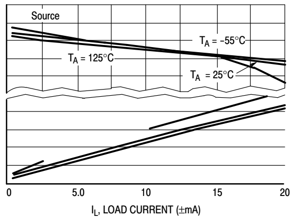
Figure 9. Split Supply Output Saturation Voltage versus Load Current
