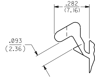
DETAIL 2 PREBENT MOUNTING EAR SCALE 4:1
