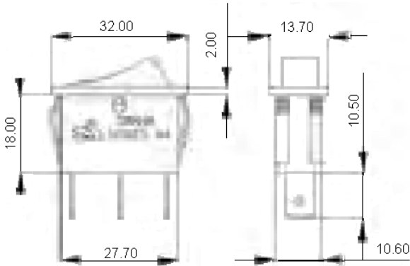
Dimensions: Millimetres
