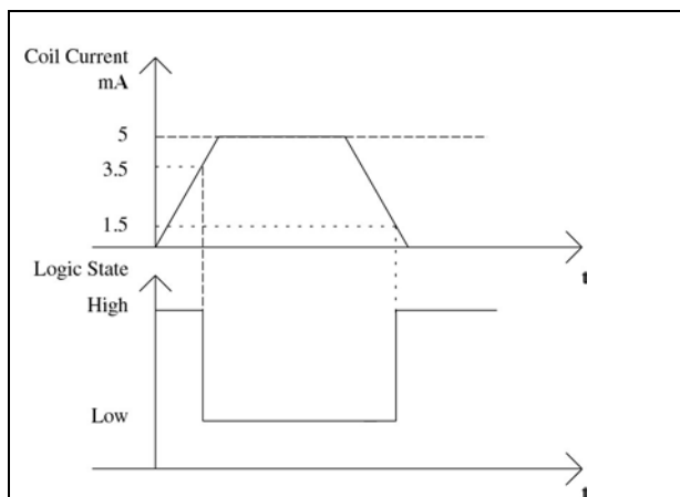
Figure 1. IL31xx Series Input Transfer Function
