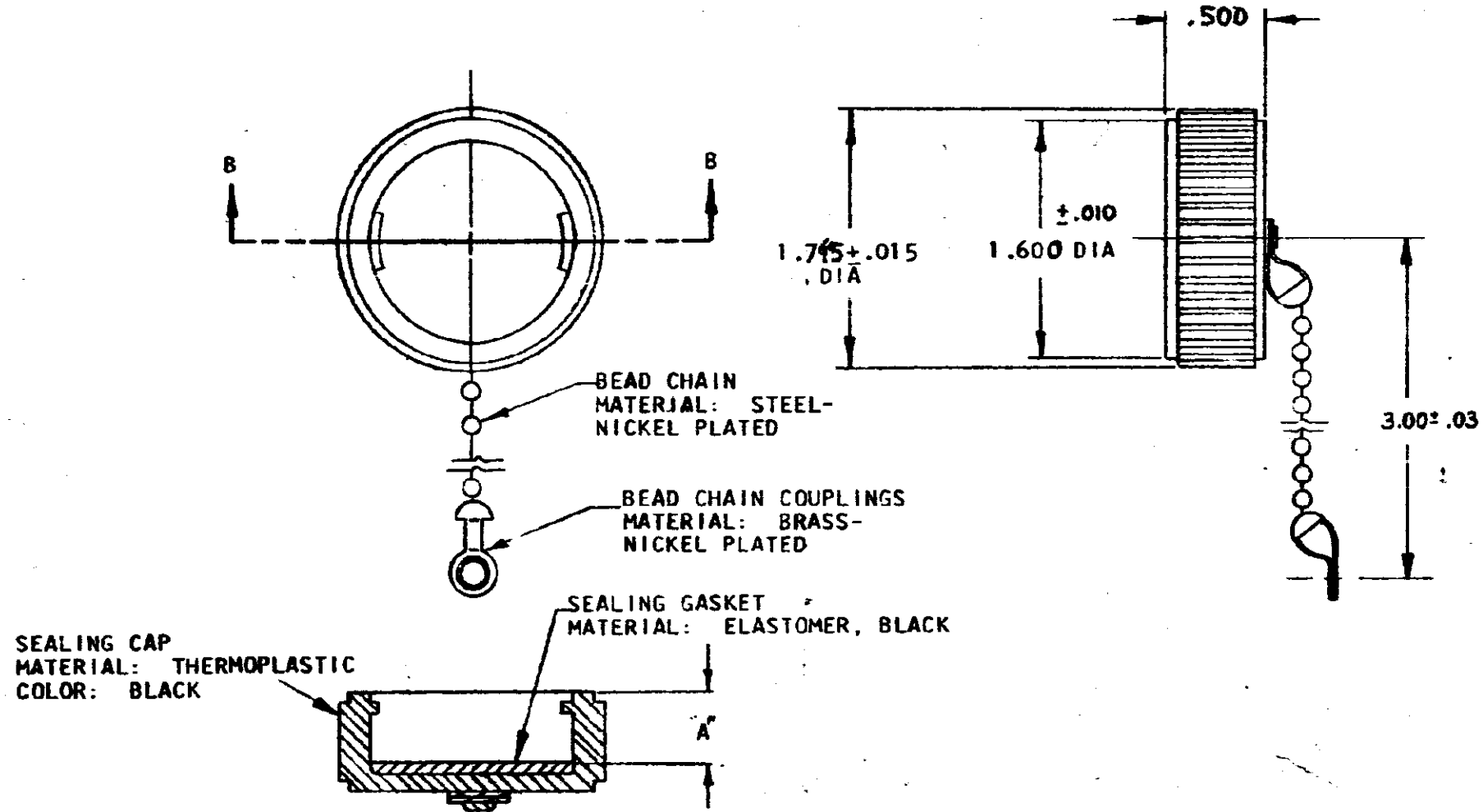
SECTION B-B
