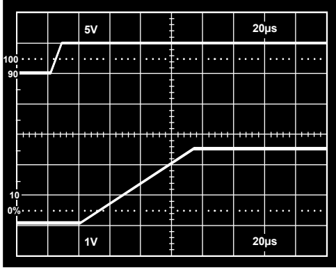
Figure 22. Turn-On Characteristics
