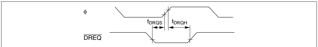
Figure 20.24 DMAC \overline{\text{DREQ}} Input Timing
