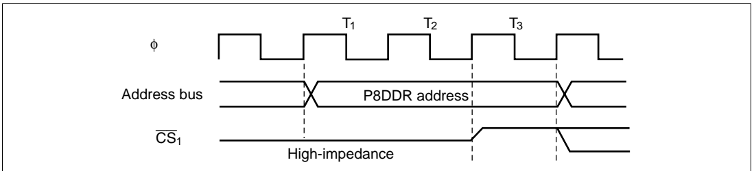
Figure 6.48 DDR Write Timing
