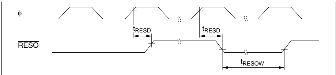
Figure 20.6 Reset Output Timing
