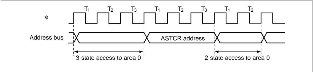
Figure 6.47 ASTCR Write Timing
