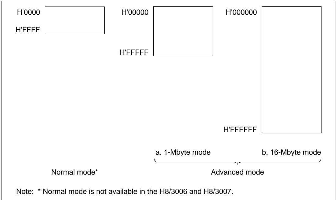
Figure 2-2 Memory Map
