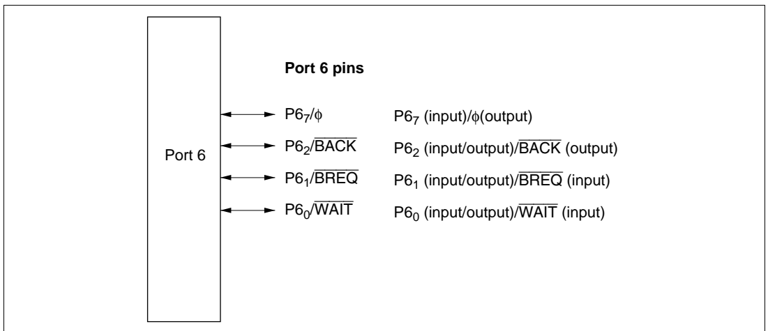
Figure 8.2 Port 6 Pin Configuration
