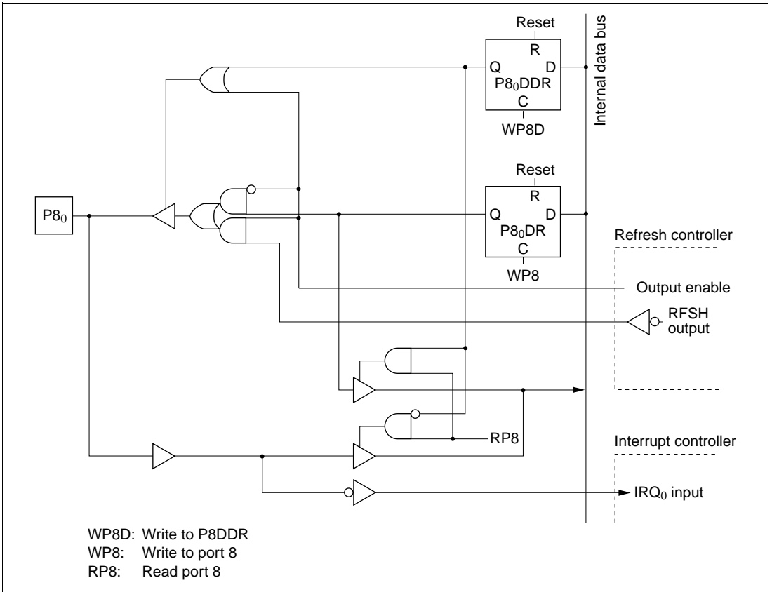
Figure C.4 (a) Port 8 Block Diagram (Pin P8 0 )
