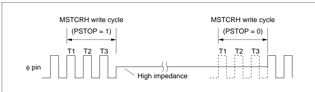
Figure 19.3 Starting and Stopping of System Clock Output
