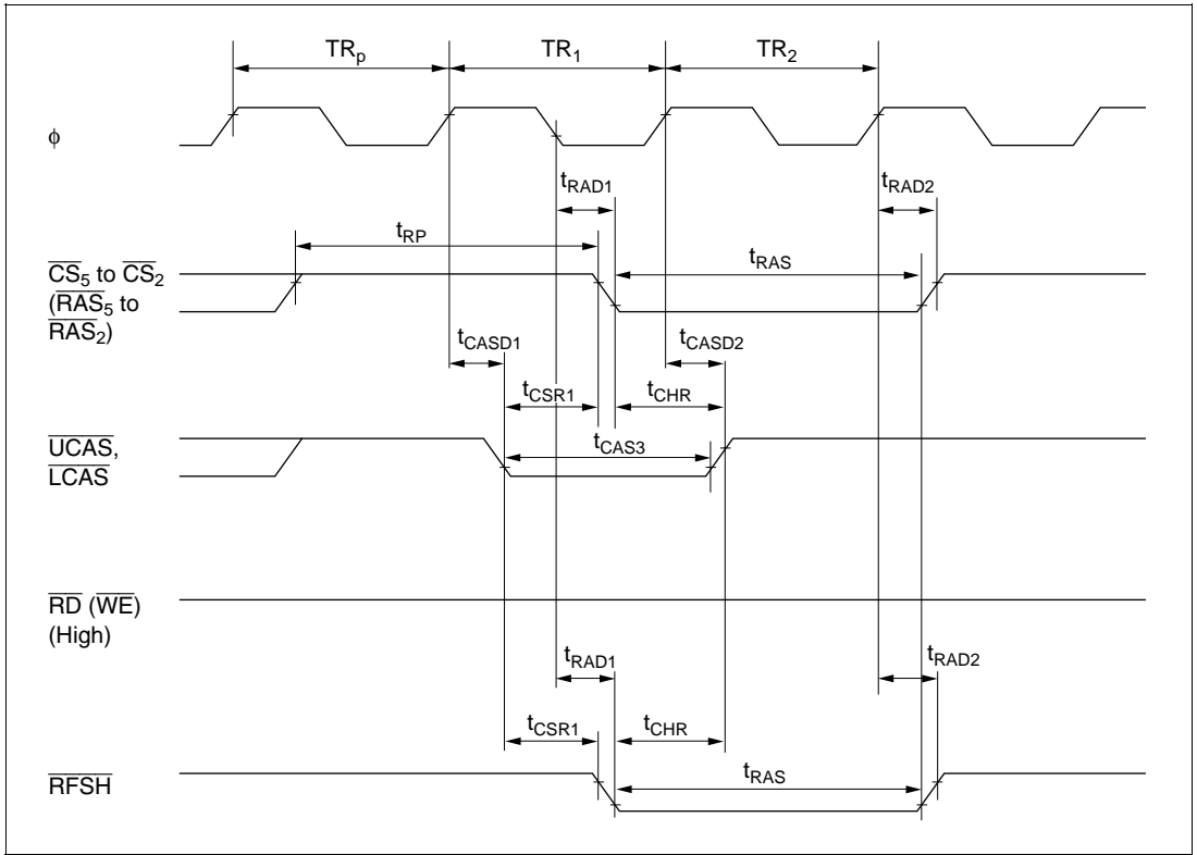
Figure 20.15 DRAM Bus Timing (CAS Before RAS Refresh)
