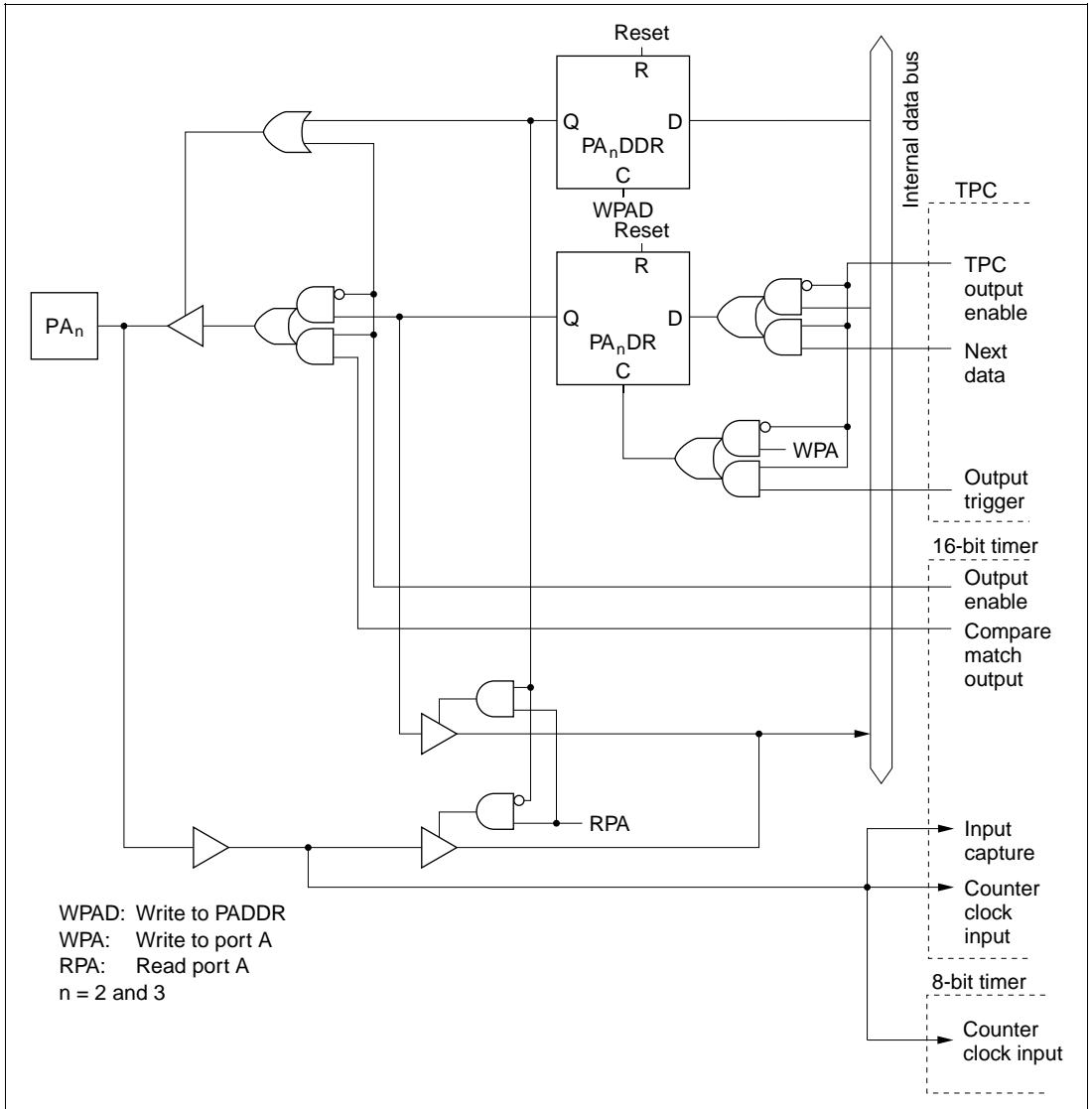
Figure C.6 (b) Port A Block Diagram (Pins PA 2 , PA 3 )
