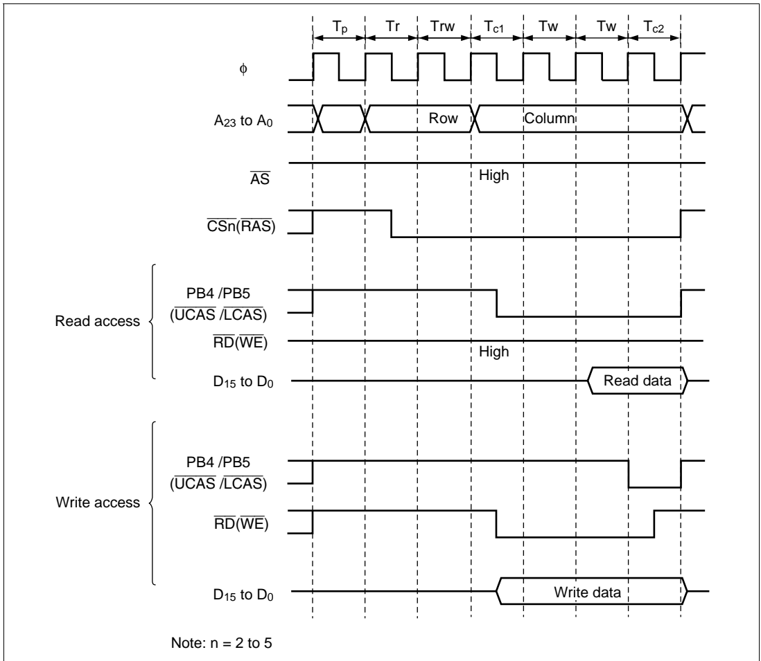
Figure 6.18 Example of Wait State Insertion Timing (CSEL = 0)
