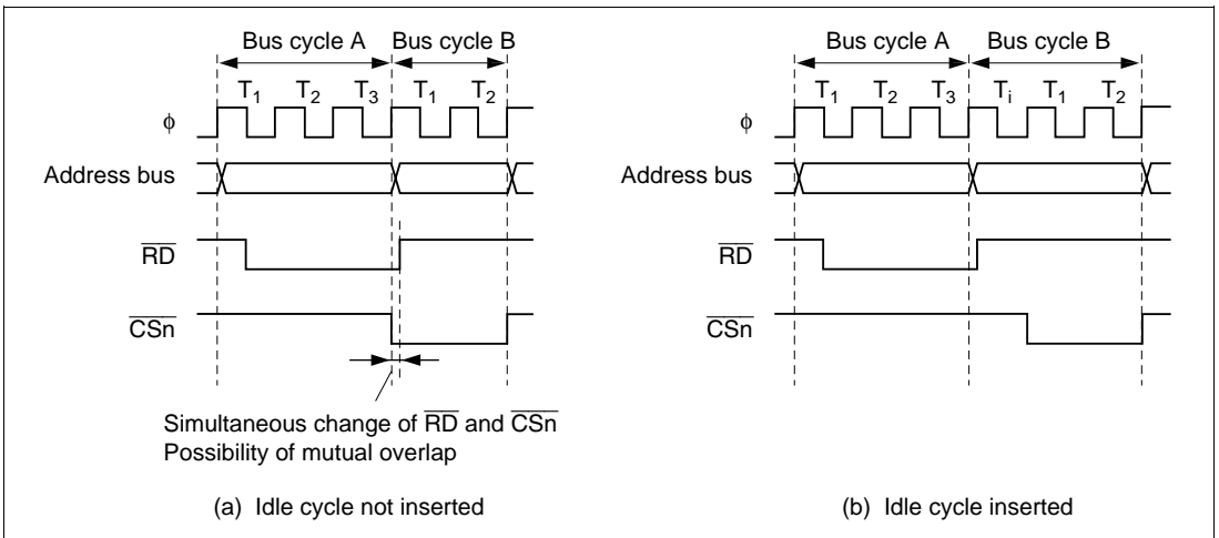
Figure 6.45 Example of Idle Cycle Operation (5)
