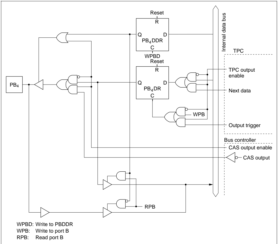
Figure C.7 (c) Port B Block Diagram (Pin PB 4 )
