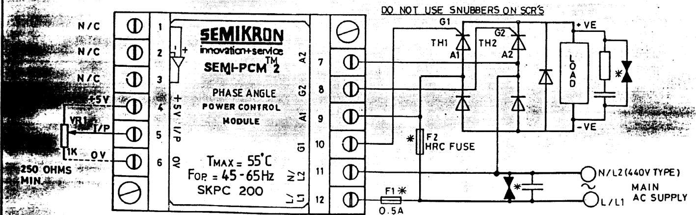
ALTERNATIVE HALF CONTROLLED D.C. BRIDGE (B2HKF).
