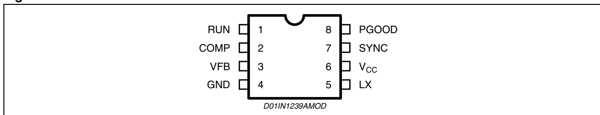
Figure 3. Pin Connection
