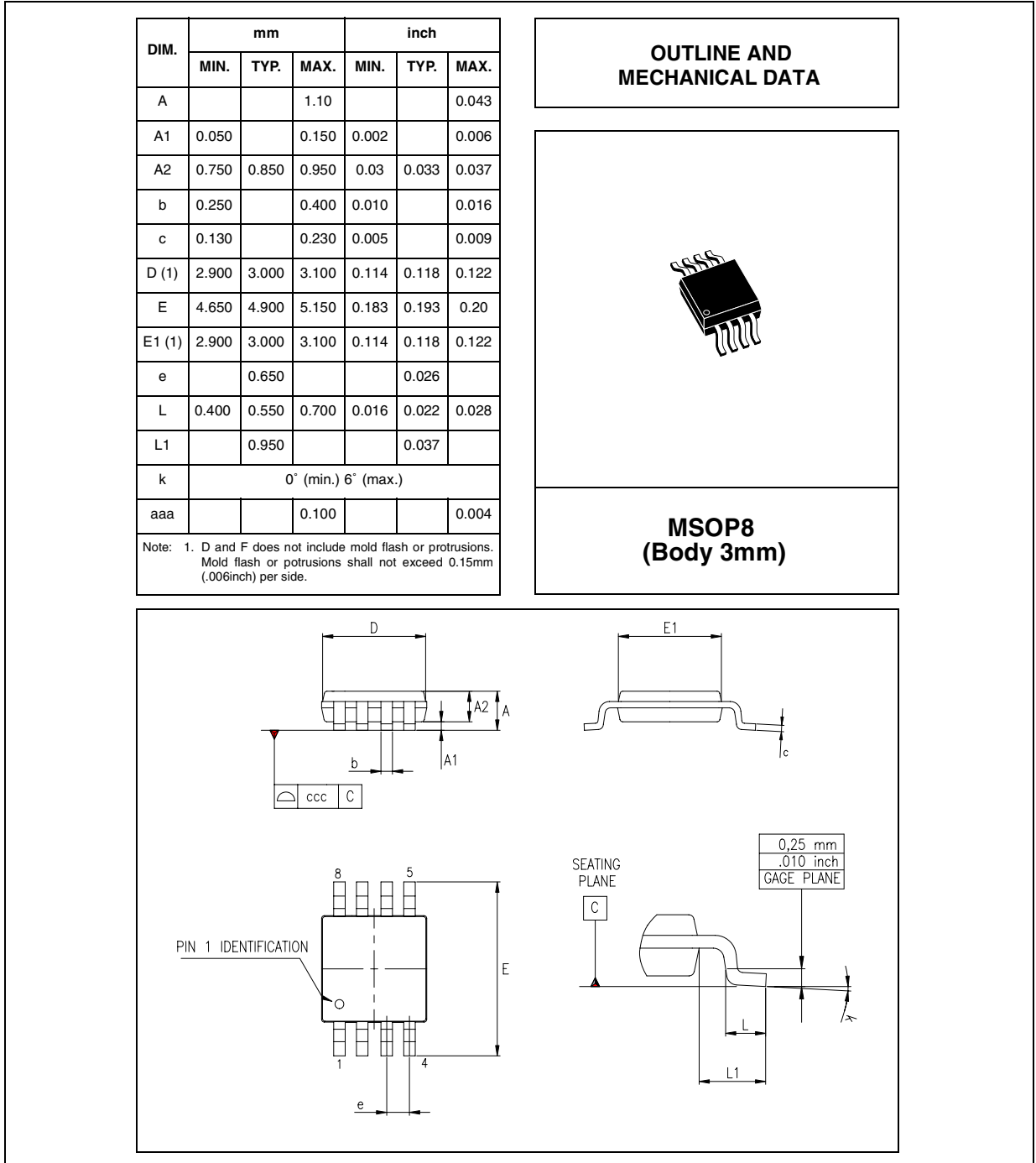
Figure 5. MSOP8 Mechanical Data & Package Dimensions
