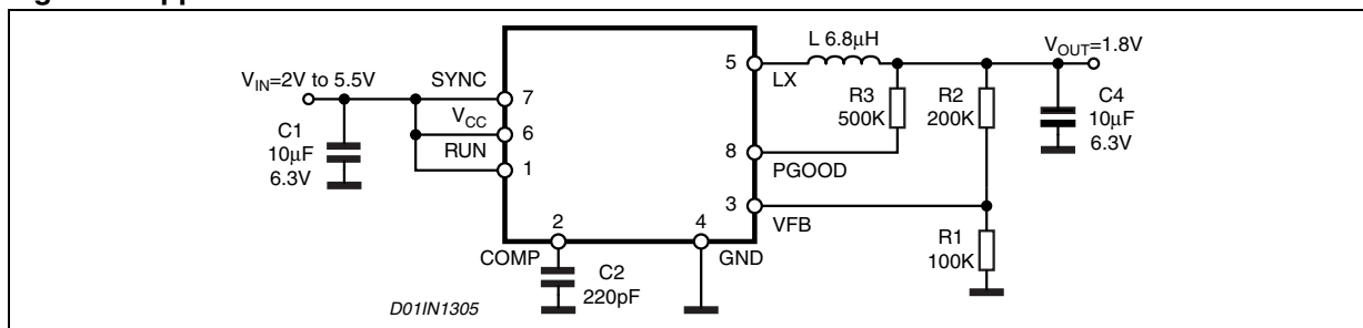
Figure 2. Application Test Circuit
