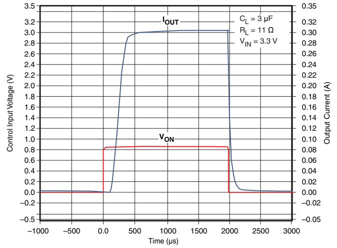
Figure 45. t_{ON} Response
