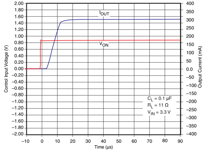
Figure 19. t_{ON} Response
