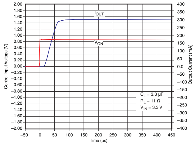
Figure 21. t_{ON} Response
