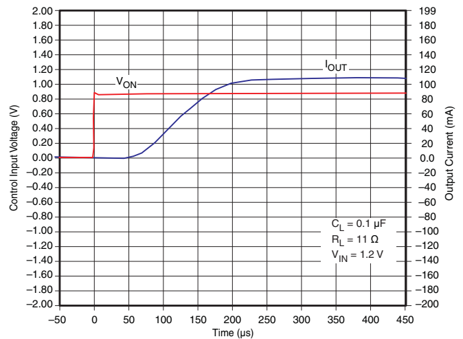
Figure 23. t_{ON} Response
