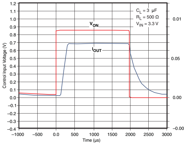
Figure 44. t_{ON} Response
