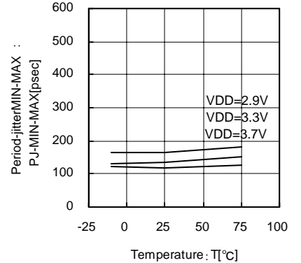
Fig.64 30MHz Temperature - Period-Jitter MIN-MAX
