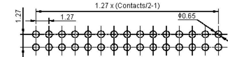
PCB Layout
