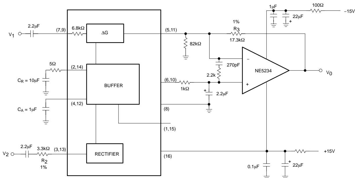
Figure 2. Test Circuit
