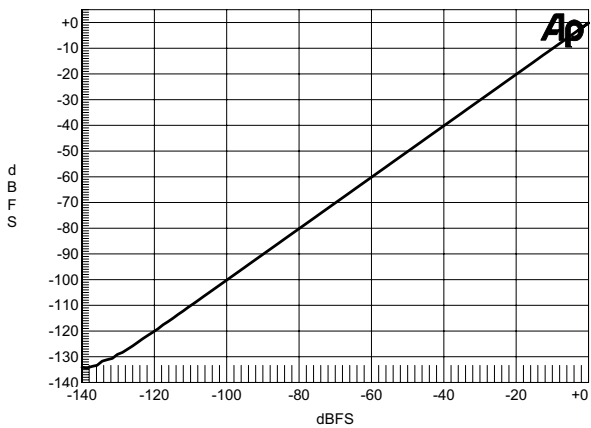
Figure 54. Linearity Error, 0 to -140 dBFS Input, 200 Hz Tone, 44.1 kHz:192 kHz
