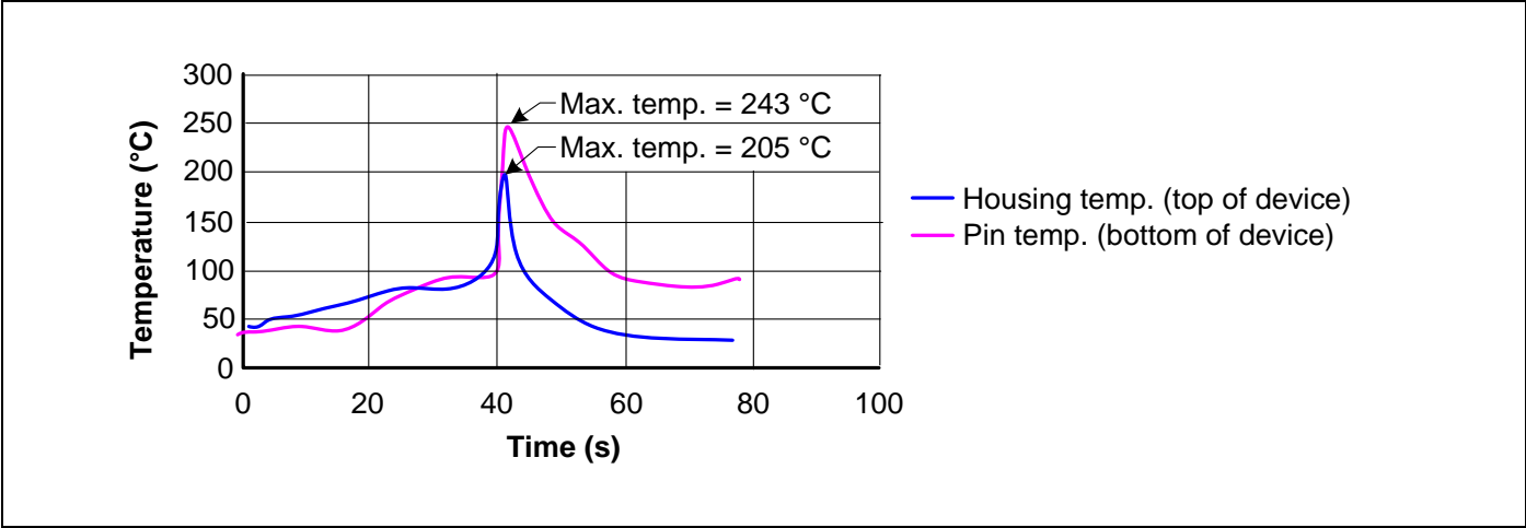
Figure 7. Wave Solder Profile
