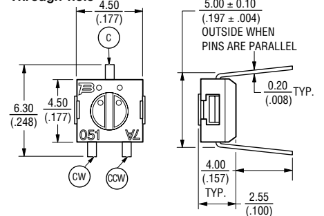
7814H Through-hole
