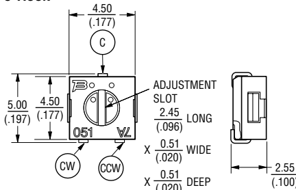
7814J J-Hook
