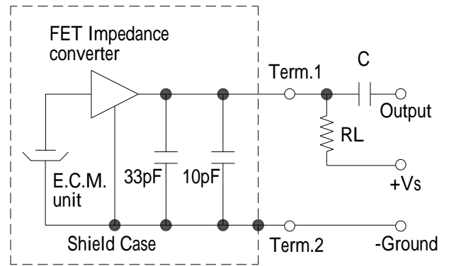
Schematic Diagram
