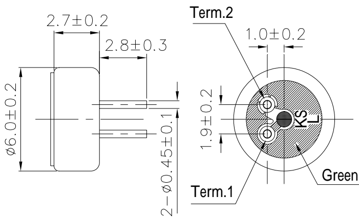
Schematic Diagram
