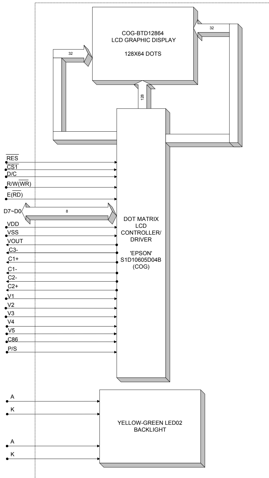
Figure 3: Block Diagram.
