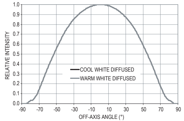
Figure 4. Radiation Pattern
