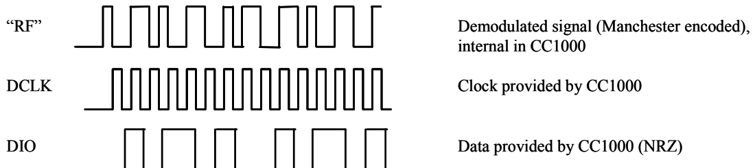
Figure 8. Synchronous Manchester encoded mode
