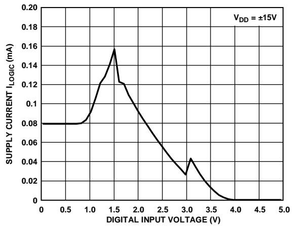
Figure 40. Supply Current I_{LOGIC} vs. Digital Input Voltage
