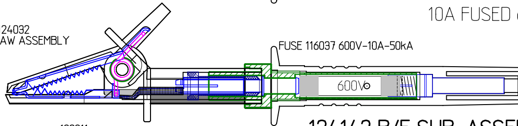
122011 LOWER JAW ASSEMBLY
