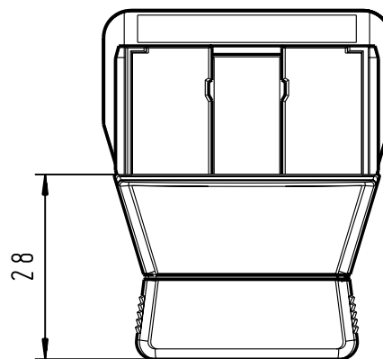
ROW-Stecker 1809281 ROW-plug 1809281
