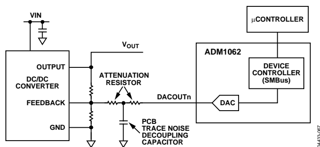
Figure 32. Open-Loop Margining System Using the ADM1062
