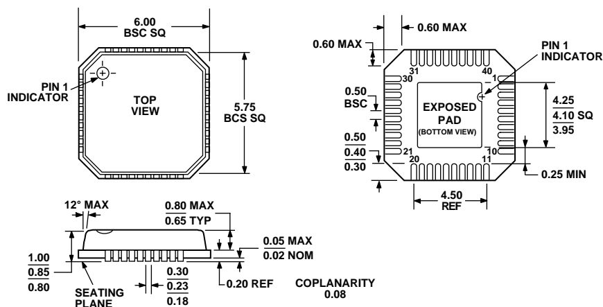
Figure 51. 40-Lead Lead Frame Chip Scale Package [LFCSP_VQ] 6 × 6 Body, Very Thin Quad (CP-40) Dimensions shown in millimeters
