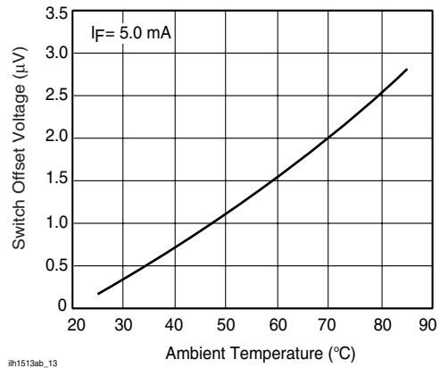
Figure 14. Switch Offset Voltage vs. Temperature
