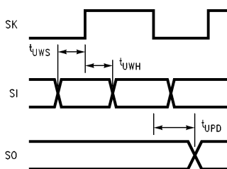
FIGURE 2. MICROWIRE/PLUS Timing
