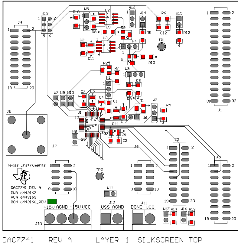
Figure 2-1. Layer One (Top Silkscreen)
