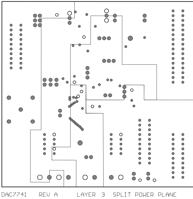
Figure 2-3. Layer 3 (Power Plane)
