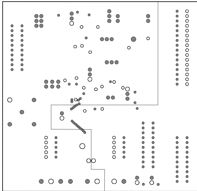
Figure 2-2. Layer Two (Ground Plane)
