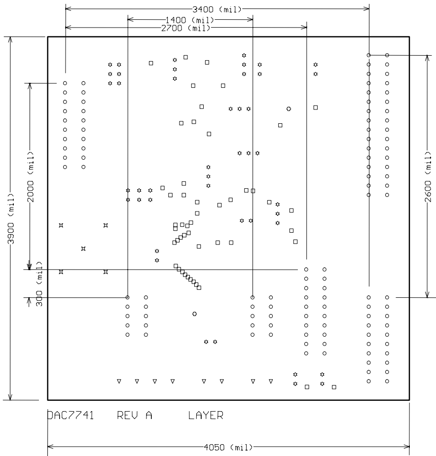
Figure 2-5. Drill Drawing
