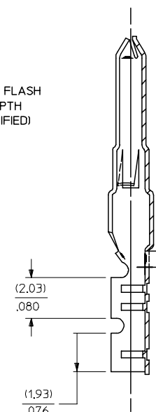
SECT. "A-A"
