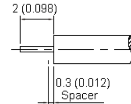
Stripping Dimension
