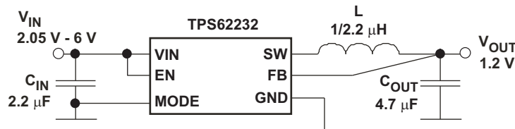
Figure 43. TPS62232 1.2V Output
