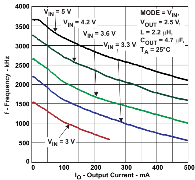
Figure 18. Switching Frequency vs Output Current, 2.5V Output Voltage MODE = VIN
