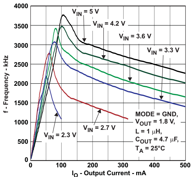
Figure 15. Switching Frequency vs Output Current, 1.8V Output Voltage MODE = GND
