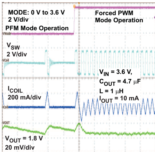
Figure 31. Mode Transition PFM / Forced PWM Mode
