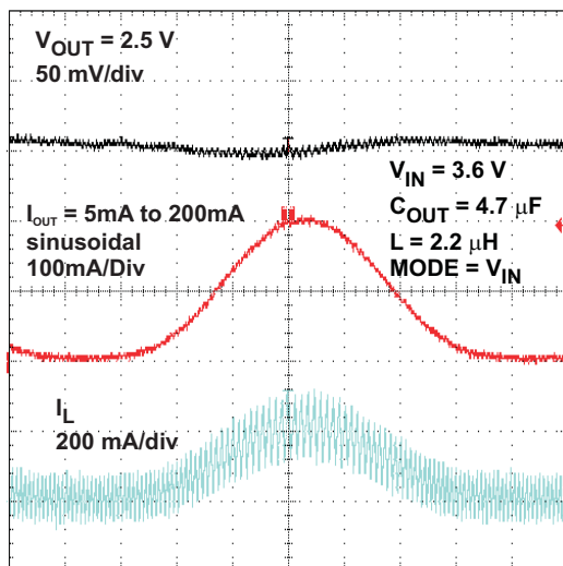
Figure 33. AC – Load Regulation Performance 2.5V V_{OUT} PWM Mode
