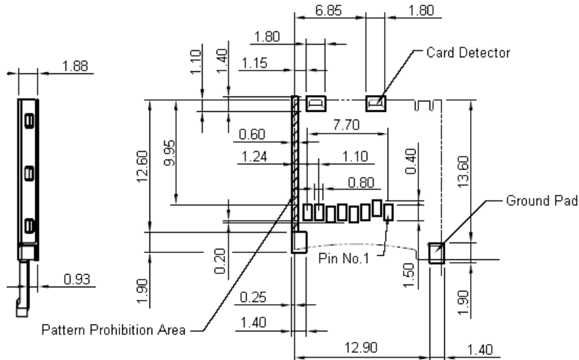
PC Board Layout (Top View)
