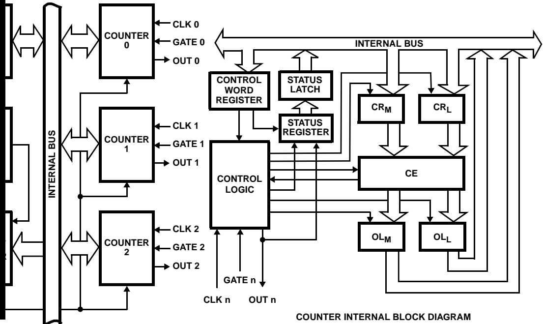
COUNTER INTERNAL BLOCK DIAGRAM
