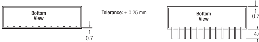
Pin Connections
