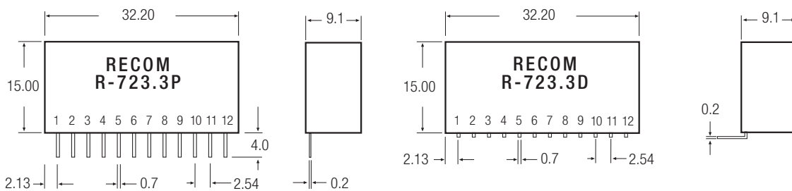
SIP12 PIN Package
