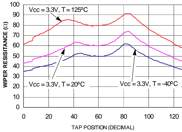
FIGURE 1. WIPER RESISTANCE vs TAP POSITION [(RW) = VCC/RTOTAL] FOR 10kΩ (W)
