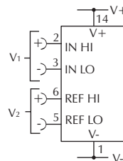
Check Link 1 is OPEN . Measuring the ratio of two voltages. Reading = 1000 V 1 /V 2 50mV < V 2 < 200mV V 1 < 2V 2 .
