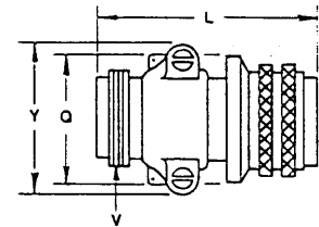
97-4106B straight plug
