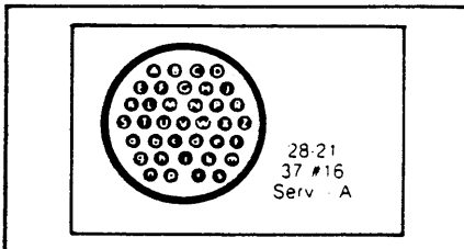
37 contacts
