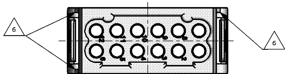
CONTACT ARRANGEMENT: VIEW FROM CONNECTING SIDE
