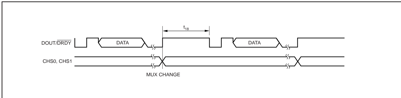
FIGURE 13. Multiplexer Operation.
