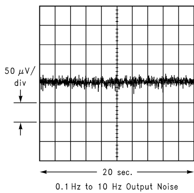
0.1Hz to 10Hz output Noise
