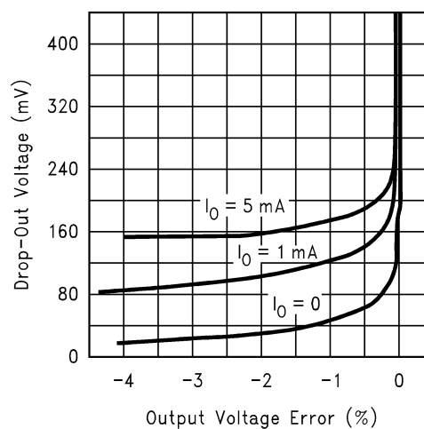
Dropout Voltage vs Output Error
