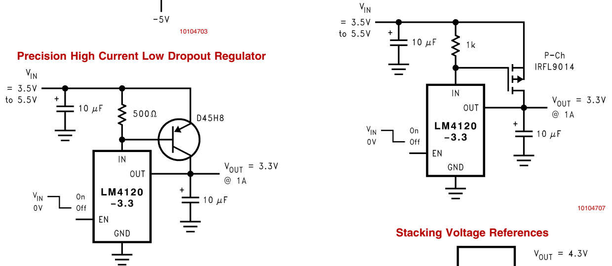
Precision High Current Low Dropout Regulator
