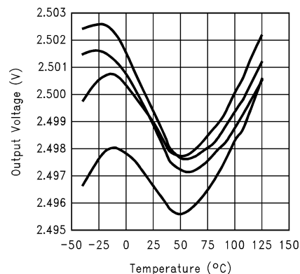
Typical Temperature Drift
