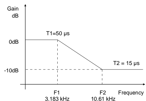
Figure 11. De-Emphasis Curve
