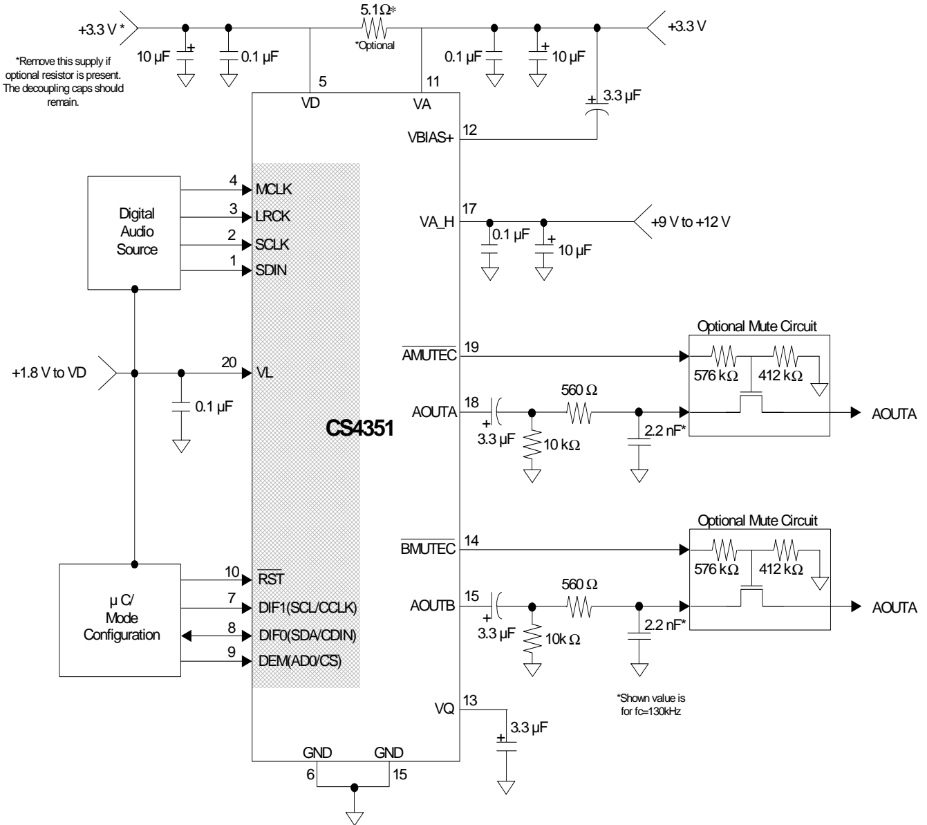
Figure 4. Typical Connection Diagram
