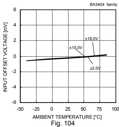
Fig. 104 Input Offset Voltage - Ambient Temperature (Vicm=0[V], VOUT=0[V])
