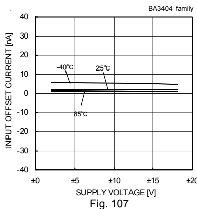
Fig. 107 Input Offset Current - Supply Voltage (Vicm=0[V], VOUT=0[V])
