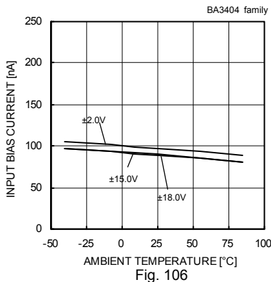
Fig. 106 Input Bias Current - Ambient Temperature (Vicm=0[V], VOUT=0[V])
