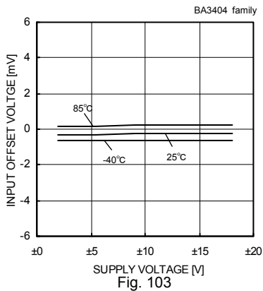
Fig. 103 Input Offset Voltage - Supply Voltage (Vicm=0[V], VOUT=0[V])
