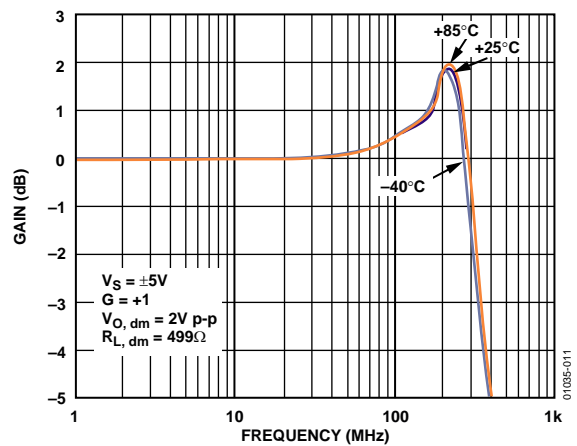
Figure 10. Large Signal Response vs. Temperature (See Figure 56)
