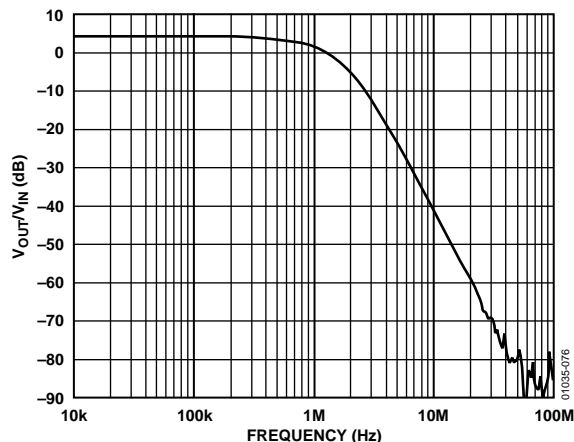
Figure 76. Frequency Response of 1 MHz Low-Pass Filter
